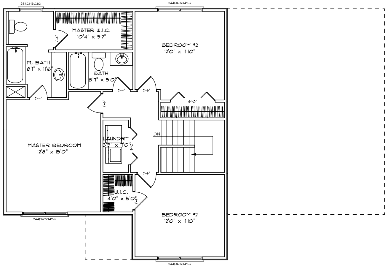
JALYN SECOND FLOOR 8' WALLS 905 S.F.
