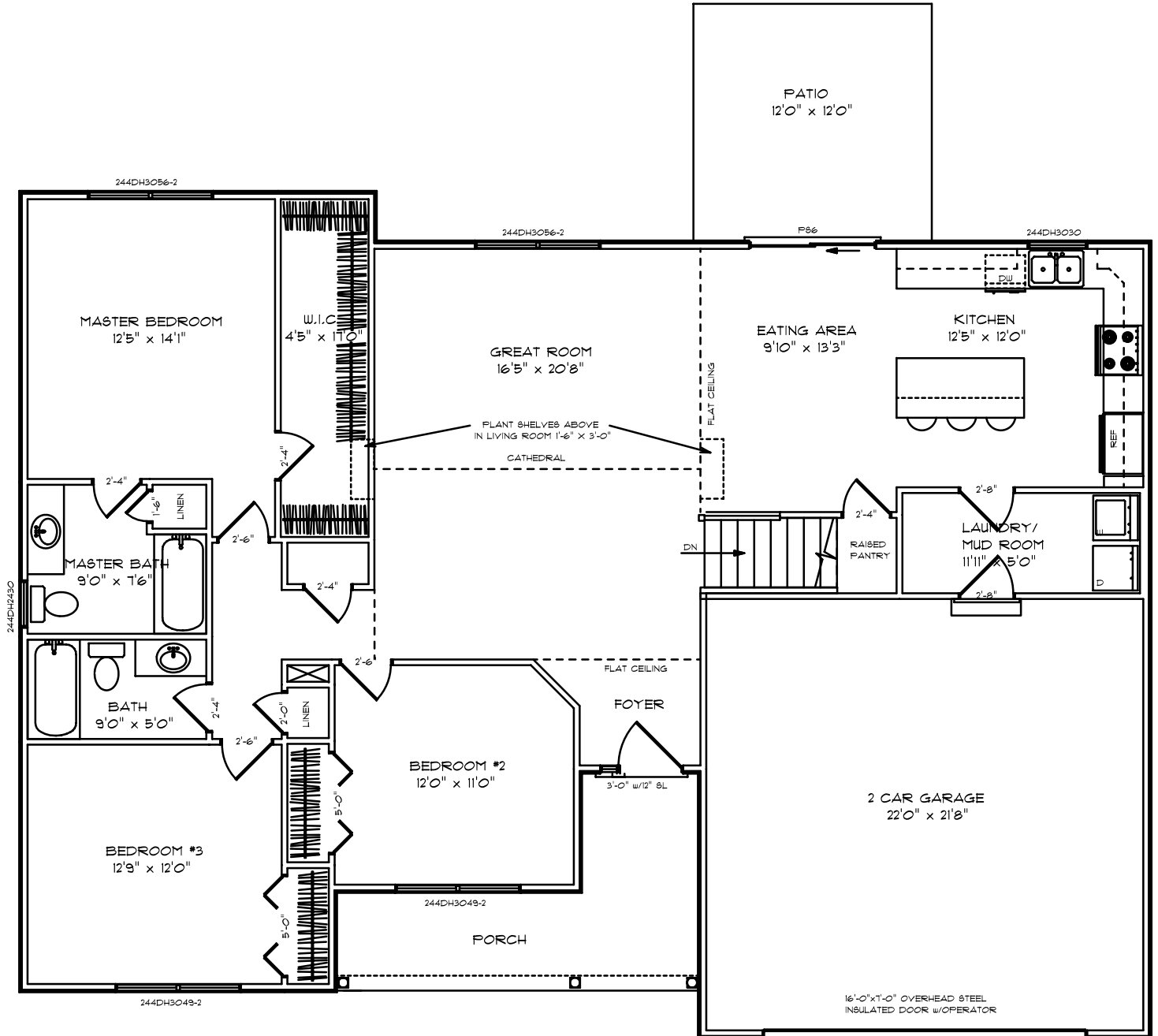
CHRISTINA MAIN 8' WALLS 1622 S.F.
