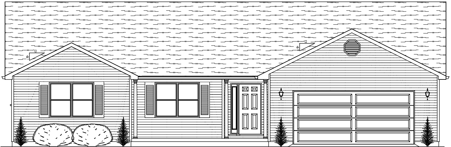
CHRISTINA FRONT ELEVATION
