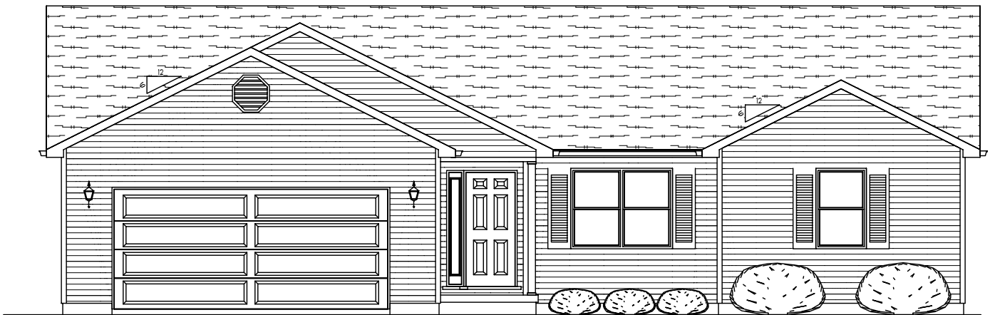
COADY FRONT ELEVATION
